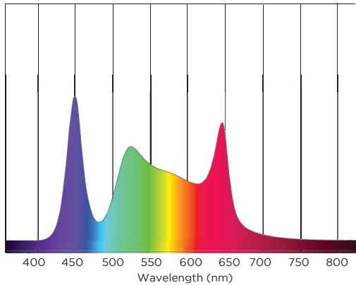
FIGURE 14. VL5LED PRODUCING 5600K WHITE
