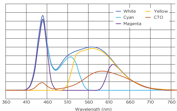
FIGURE 3. WHITE LED FIXTURE WITH FILTERS
