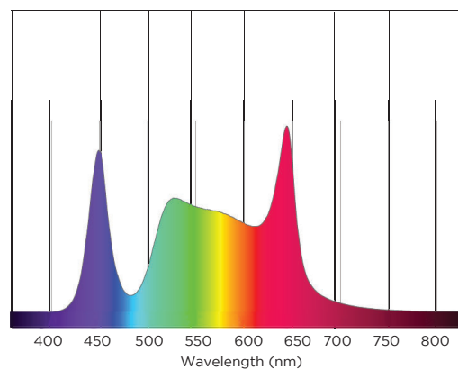
FIGURE 13. VL5LED PRODUCING 4500K WHITE
