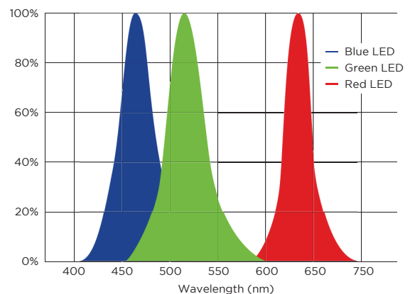
FIGURE 4. ILLUSTRATION OF RGB LEDS 1
