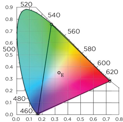
FIGURE 5. CIE 1931 COLOR SPACE
