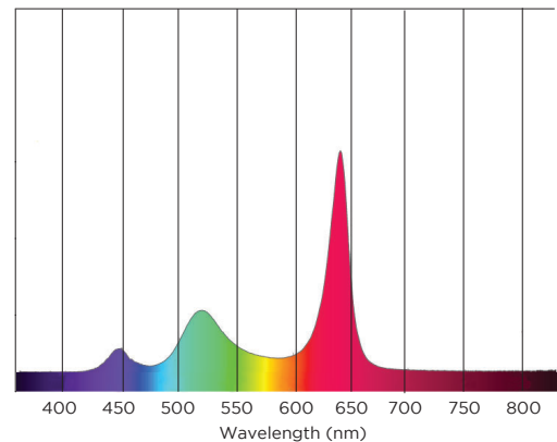
FIGURE 7. RGBW FIXTURE AT 3000K WHITE
