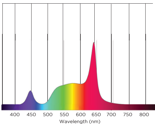
FIGURE 12. VL5LED PRODUCING 2700K WHITE
