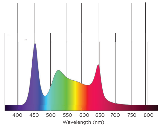
FIGURE 10. VL5LED AT 6500K WHITE
