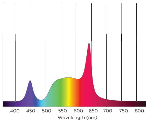
FIGURE 9. VL5LED AT 3200K WHITE
