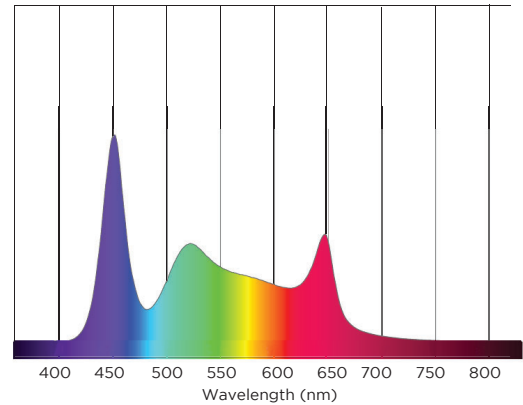
FIGURE 15. VL5LED PRODUCING 8000K WHITE
