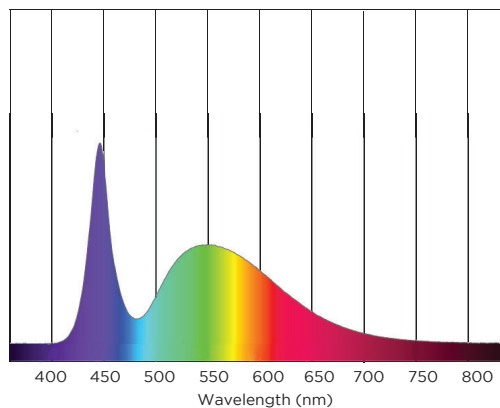
FIGURE 8. RGBW FIXTURE AT 6500K WHITE
