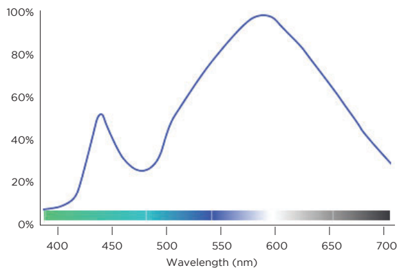
FIGURE 6. SPECTRUMS OF TYPICAL WHITE PHOSPHOR LED 2
