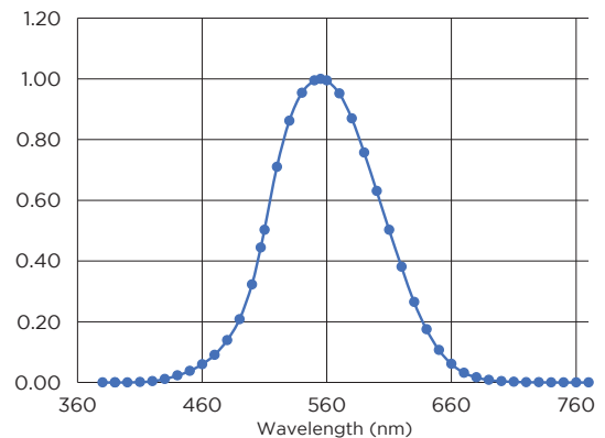
FIGURE 1. EYE SENSITIVITY CURVE ACCORDING TO CIE
