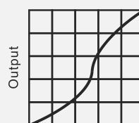
S-curve
